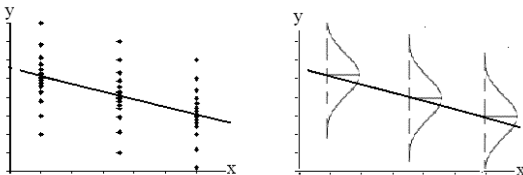
Figure 3.15: The y values for each x value are normally distributed about the line with the same standard deviation. For each x value, the mean of the y values lies on the regression line. More y values lie near the line than are scattered further away from the line.
