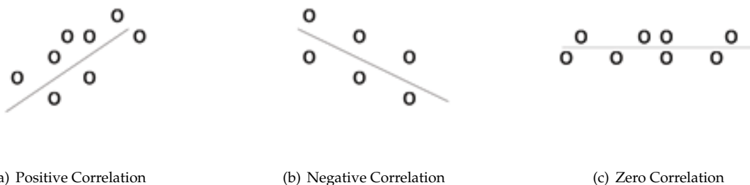
Figure 3.11: (a) A scatter plot showing data with a positive correlation. 0 < r < 1 (b) A scatter plot showing data with a negative correlation. -1 < r < 0 (c) A scatter plot showing data with zero correlation. r=0
