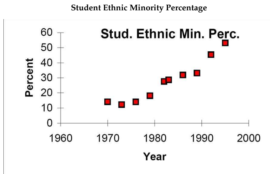
Figure 13.6: By hand, verify the scatterplot above.
