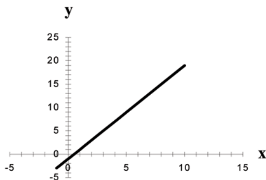
Figure 3.1: Graph of the equation y = -1 + 2x .
